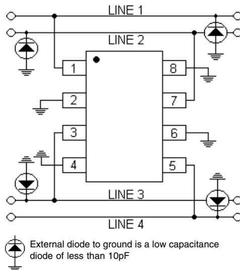
Figure 1. Unidirectional Common-Mode Protection
